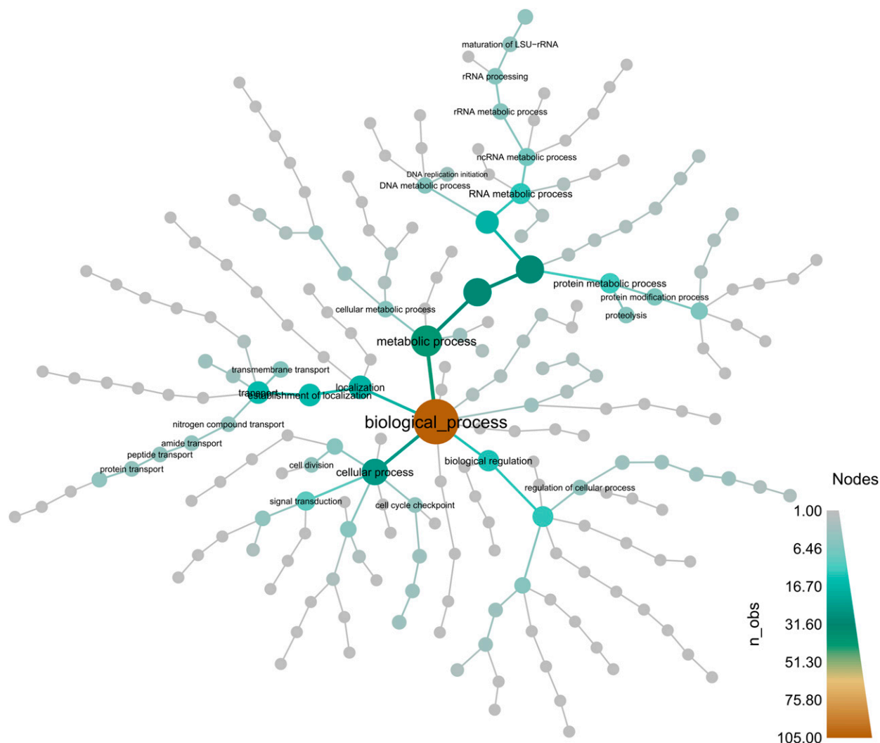
Figure 4 Composition and hierarchical organization of GO terms associated to the 675 genes with consistent sex-biased gene expression in all three species. n_{obs} : number of genes in the given GO category.
