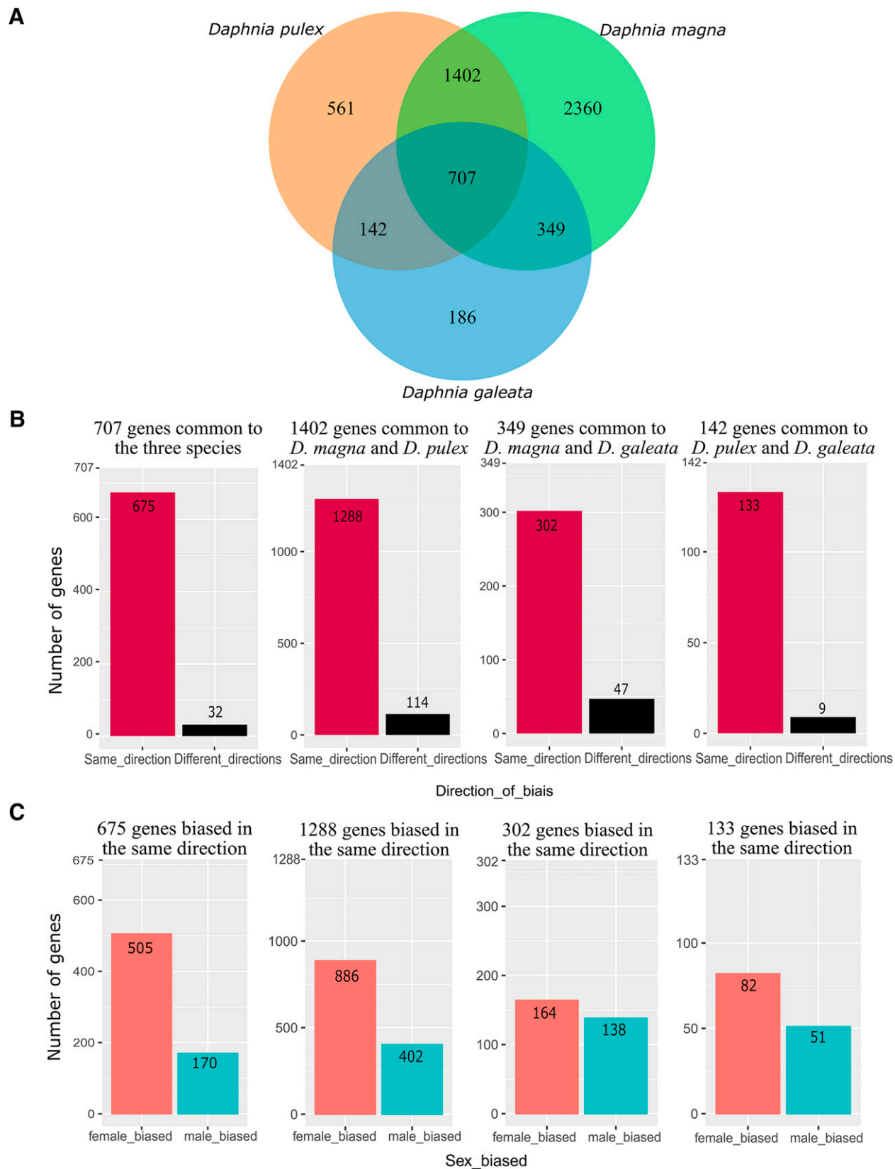
Figure 2 A. Venn diagram showing the number of sex-DE genes among the 7453 one-to one orthologs in each of the three species of Daphnia . B. Number of sex-DE genes being biased in the same vs. opposite directions. Panels from left to right: genes being sex-DE all three species (707 genes), genes being sex-DE only in D. magna and D. pulex (1402 genes), D. magna and D. galeata , (349 genes), and D. pulex and D. galeata (142 genes). C. Number of female-biased and male-biased genes in each of the four categories depicted in Figure 2 B. (only genes being biased in the same direction).
